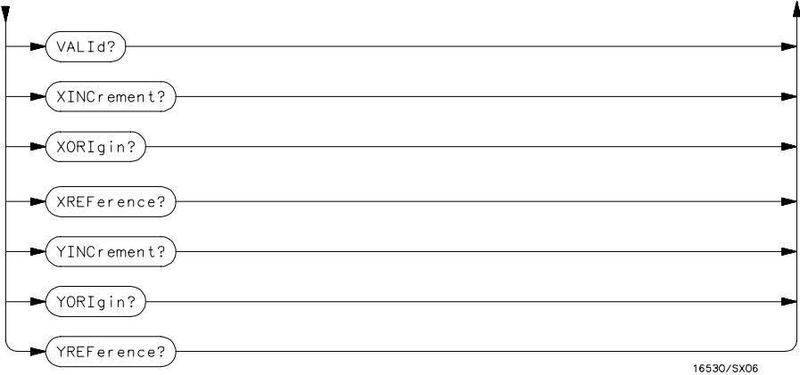
WAVEform Subsystem Syntax Diagram (Continued)
